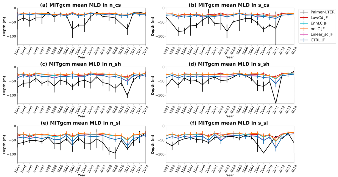
Figure 3. Averaged mixed layer depth (MLD) for January and February each year from the Palmer-Long Term Ecological Research (LTER) cruise (black lines) and from the simulations (other colors). For the model data, the vertical lines indicate the standard deviation of the data considered in each subregion and year; for the Palmer-LTER data, the vertical lines represent the standard deviation of the data in each subregion for each cruise. Data are shown for (a) northern coast, (b) southern coast, (c) northern shelf, (d) southern shelf, (e) northern slope, and (f) southern slope.
