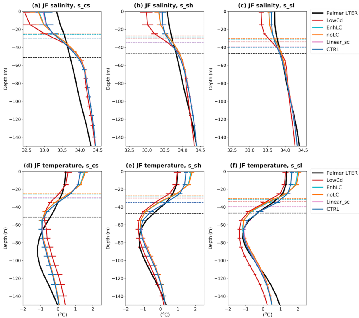
Figure 6. Simulated January–February climatology and Palmer–Long Term Ecological Research (LTER) cruise climatology of salinity for (a) southern coast, (b) southern shelf, and (c) southern slope regions, and simulated January–February climatology and Palmer–LTER cruise climatology of temperature for (d) southern coast, (e) southern shelf, and (f) southern slope regions. The horizontal solid lines represent standard deviation, and the horizontal dashed lines indicate climatological mixed layer depth for the period considered.
