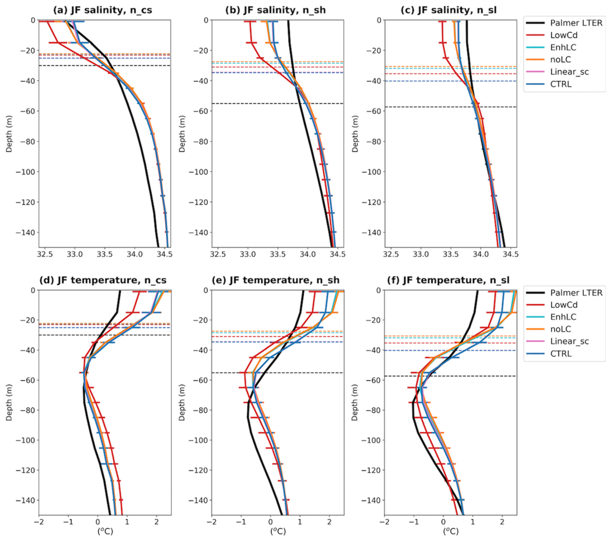
Figure 5. Simulated January–February climatology and Palmer–Long Term Ecological Research (LTER) cruise climatology of salinity for (a) northern coast, (b) northern shelf, and (c) northern slope regions, and simulated January–February climatology and Palmer–LTER cruise climatology of temperature for (d) northern coast, (e) northern shelf, and (f) northern slope regions. The horizontal solid lines represent standard deviation, and the horizontal dashed lines indicate climatological mixed layer depth for the period considered.
