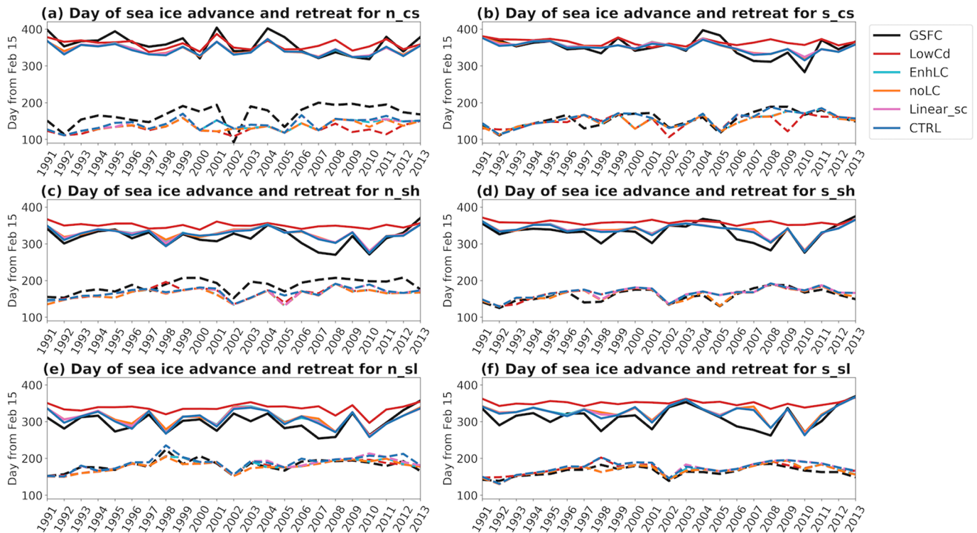
Figure 2. Evolution of the onset times of sea ice advance (dashed line) and retreat (solid) in subregions (a) northern coastal, (b) southern coastal, (c) northern shelf, (d) southern shelf, (e) northern slope, and (f) southern slope. The black lines represent results for satellite observations, and other lines represent results from different simulations.
