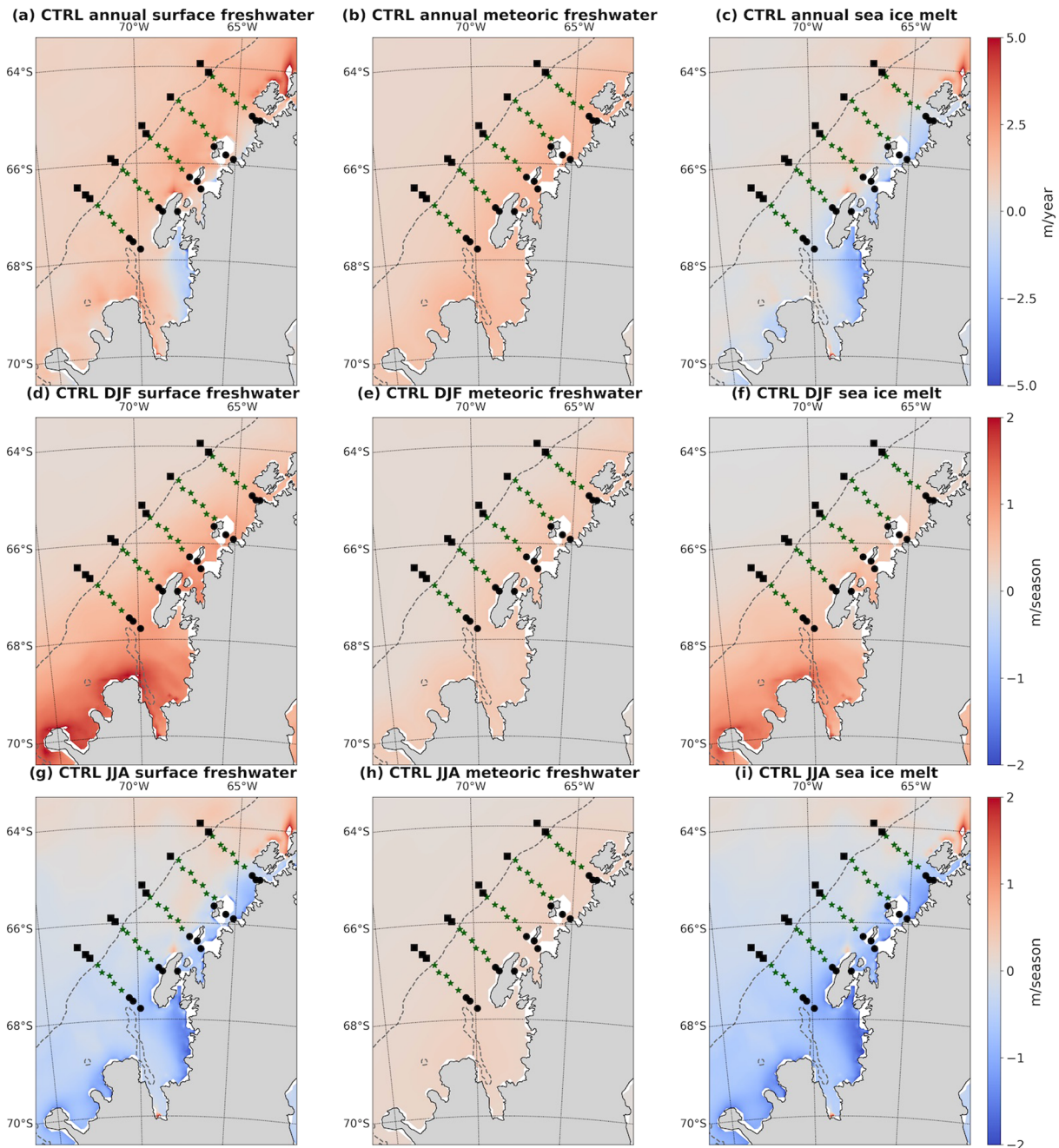
Figure 8. Annual climatology of fluxes (a–c) of total freshwater (a, d, and g), meteoric freshwater (b, e, and h), and sea ice melt (c, f, and i); summer (December–February) climatology of fluxes (d–f); and winter (June–August) climatology of fluxes (g–i). The dashed lines represent 750-m isobath, taken to be the edge of the continental shelf, and the different symbols represent coastal (black dots), shelf (green), and slope (black diamonds) stations.
