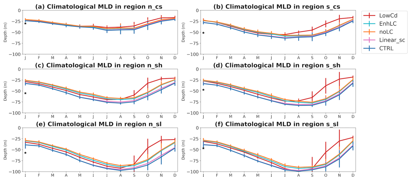
Figure 4. Simulated monthly climatologies of mixed layer depth (MLD) in (a) northern coast, (b) southern coast, (c) northern shelf, (d) southern shelf, (e) northern slope, and (f) southern slope regions. The black star in January represents the average observed MLD for each region, calculated using the Palmer-Long Term Ecological Research (LTER) cruise data.
