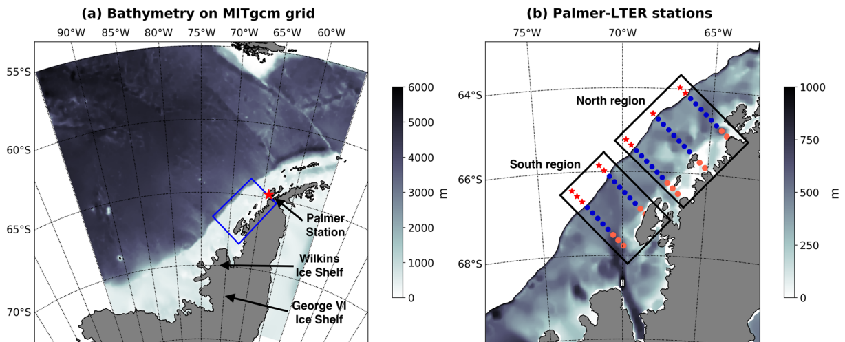
Figure 1. (a) Model bathymetry with the region of Palmer-LTER cruises marked in the blue rectangle and (b) locations of the Palmer-LTER cruise coastal (orange dots), shelf (blue dots), and slope (red stars) sampling station. The transect lines in the southern region are lines 200 (southernmost) and 300, and the transect lines in the northern region are 400, 500, and 600 (northernmost). Subregions analyzed are named northern coastal (n_cs), northern shelf (n_sh), northern slope (n_sl), southern coastal (s_cs), southern shelf (s_sh), and southern slope (s_sl).
