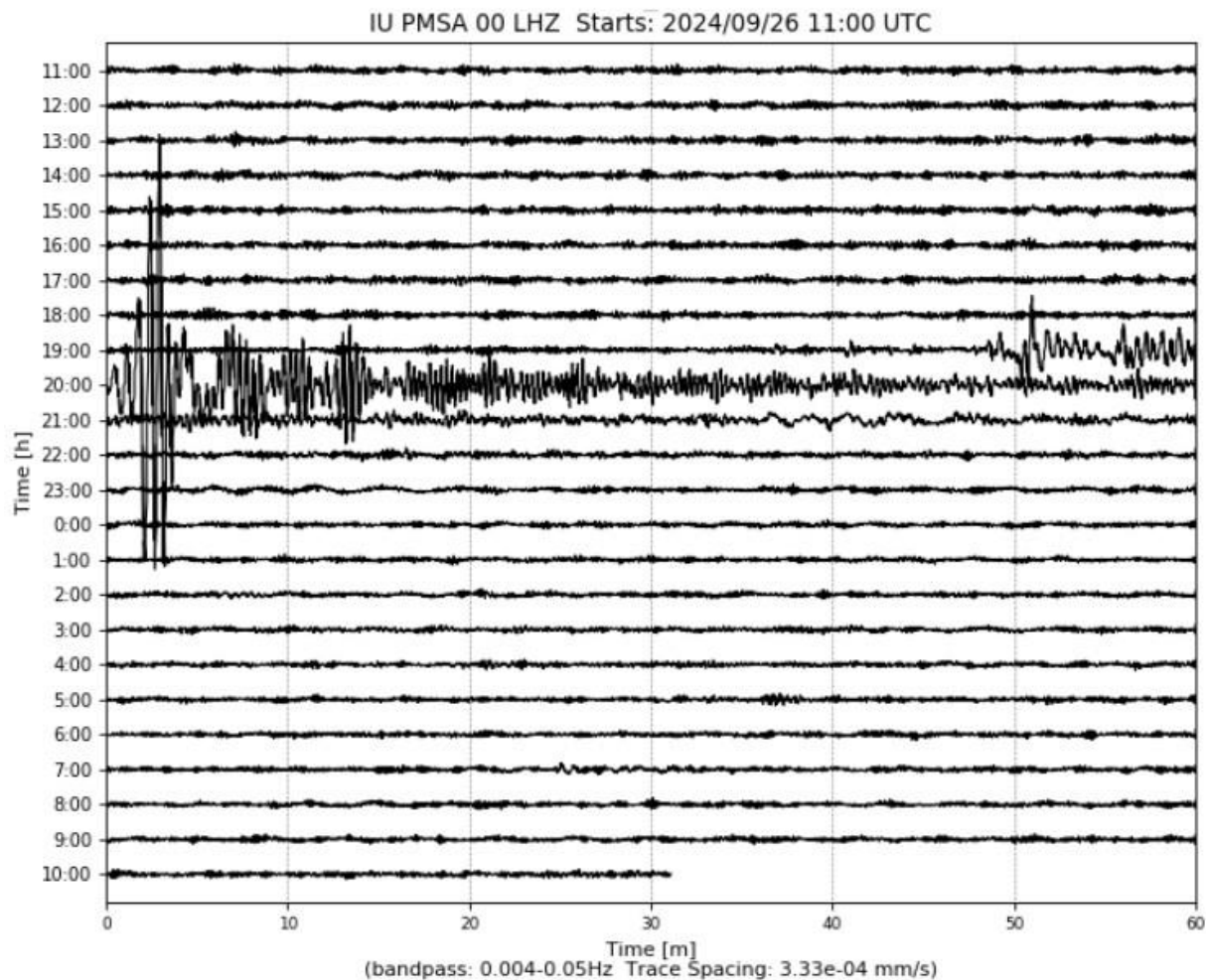
Figure 2. The September 26th 6.3 earthquake in the Mauritius – Reunion region, as recorded from the Palmer seismic station.
