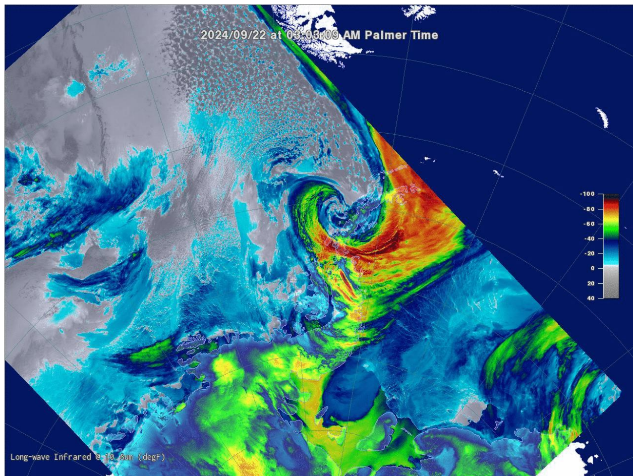
Figure 7. NOAA-Terascan September 22 nd satellite pass during our season record peak wind speed (80 knots).
