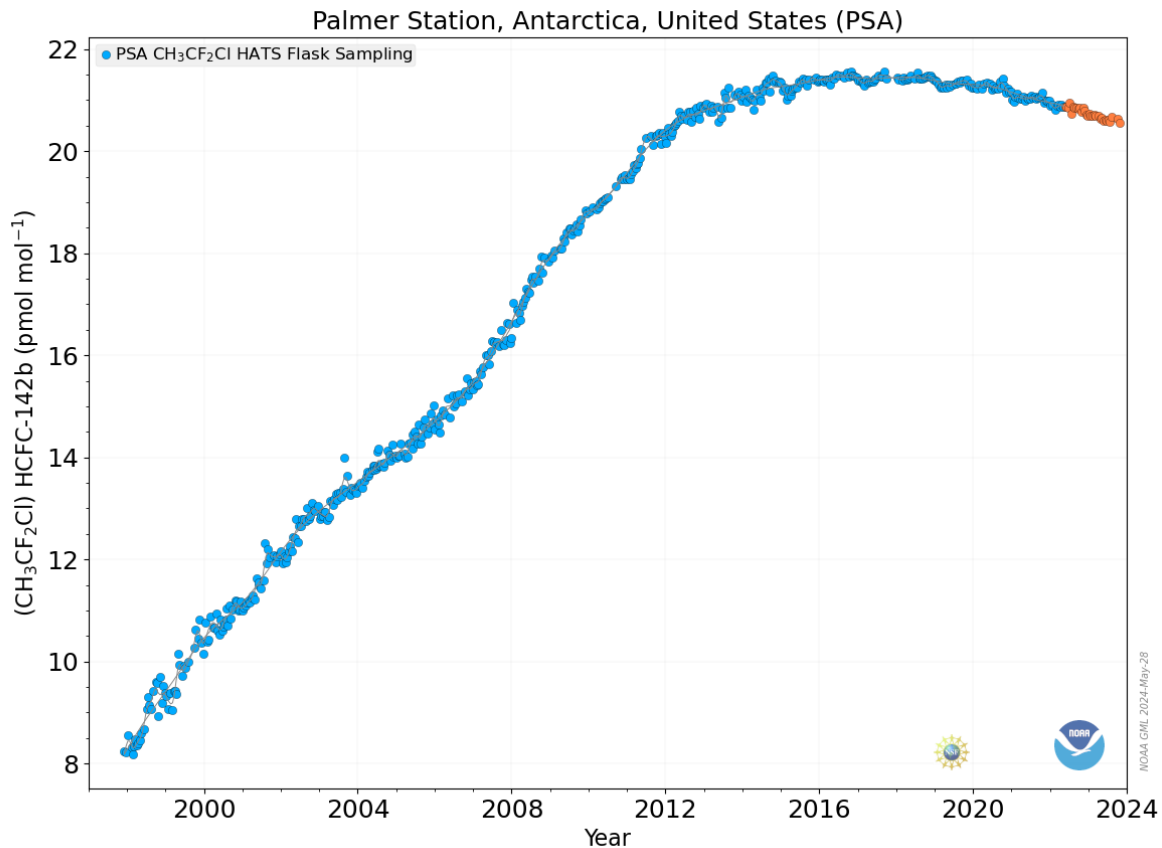
Figure 5. Hydrochlorochlorocarbon-142b ( \text{CH}_3\text{CF}_2\text{Cl} ) levels at Palmer Station dating back to 1998, one of the Halocarbon and Trace Gases measured at Palmer Station. Orange dots are preliminary data.
