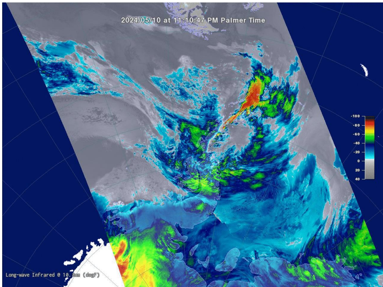
Figure 7. NOAA-19 May 10 th satellite pass during a notable snow storm.
