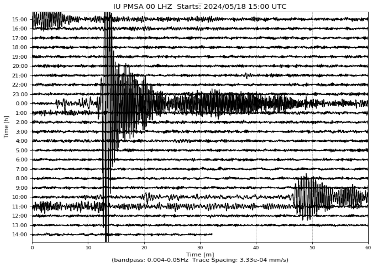
Figure 2. The May 19th 6.0 earthquake near the Aleutian Islands, Alaska, as recorded from the Palmer seismic station.
