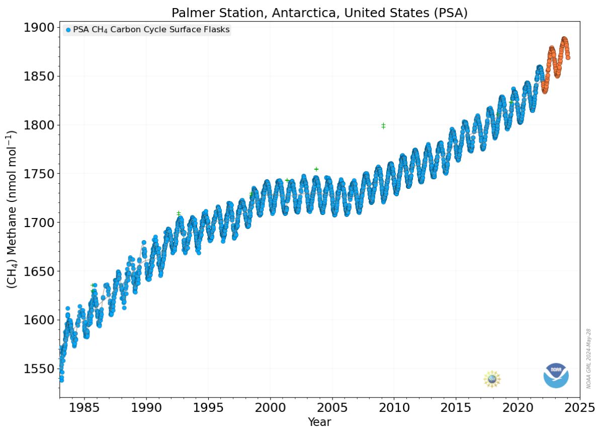
Figure 4. Methane ( CH_4 ) levels at Palmer Station dating back to 1983. Orange dots are preliminary data and green pluses are poorly mixed air masses, which should not indicate background conditions.
