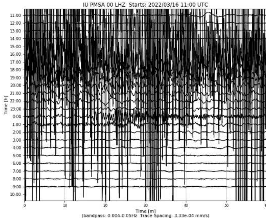
Figure 3- Honshu, Japan 7.3 Magnitude Earthquake on March 16, 2022
