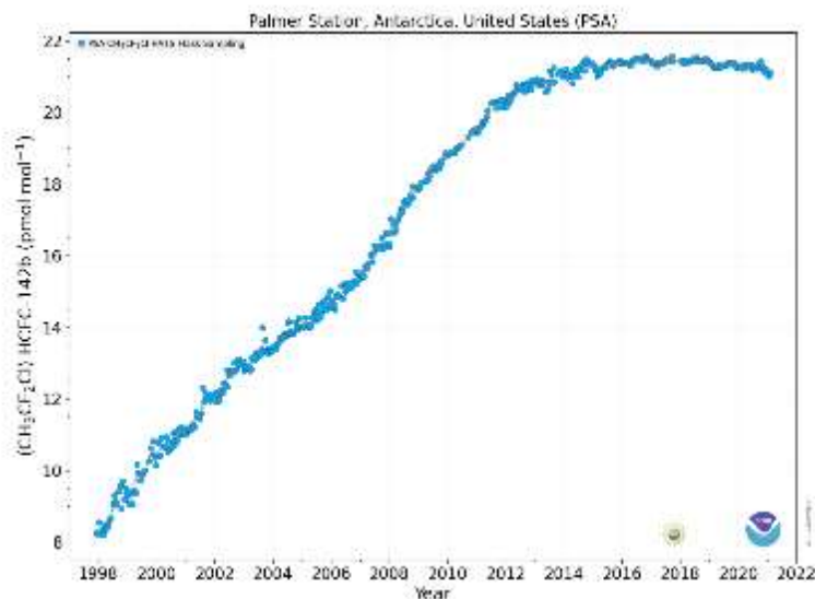
Figure 6- HCFC 142b (CH 3 CF 2 CL) Levels at Palmer Station dating back to 1998, one of the Halocarbon and Trace Gases measured at Palmer Station. Orange dots are preliminary data.
