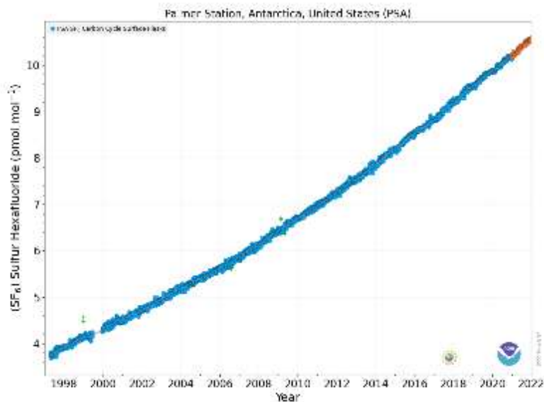
Figure 5- Sulfur Hexafluoride (SF 6 ) Levels at Palmer Station dating back to 1997. Orange dots are preliminary data.
