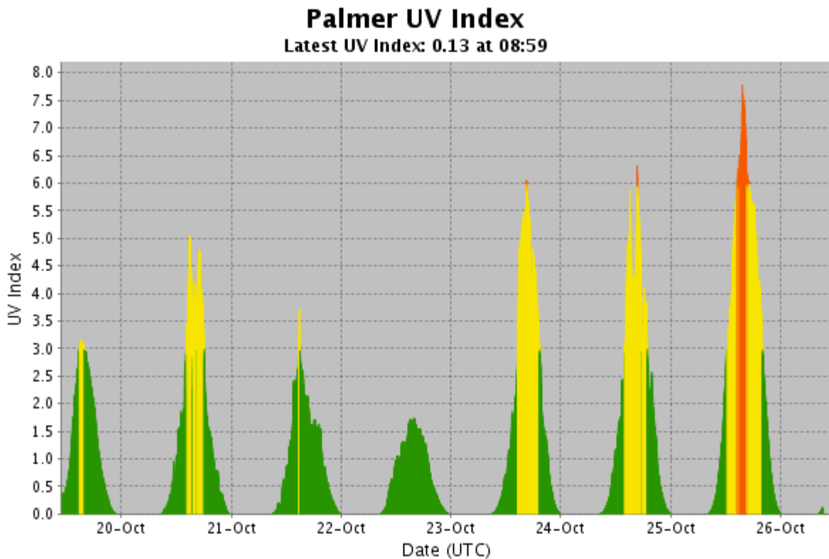
Figure 6- UV index generated from the GU-511 radiometer in real time.
