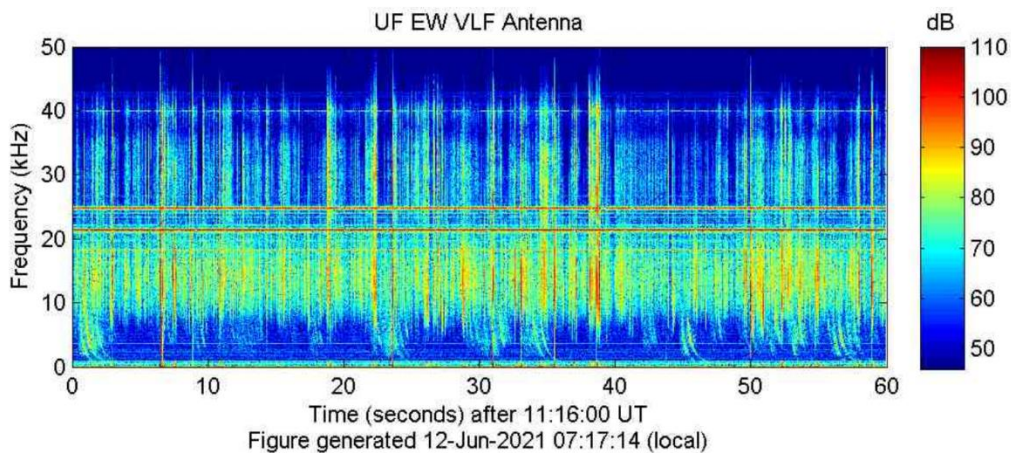
Figure 1- Real-Time broadband VLF Spectrogram from Palmer Station, Antarctica
