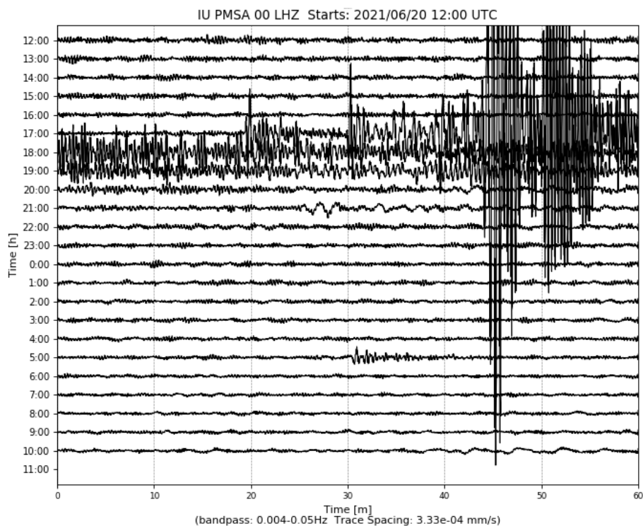
Figure 2- 6.3 Magnitude earthquakes near the east coast of New Zealand on June 20, 2021
