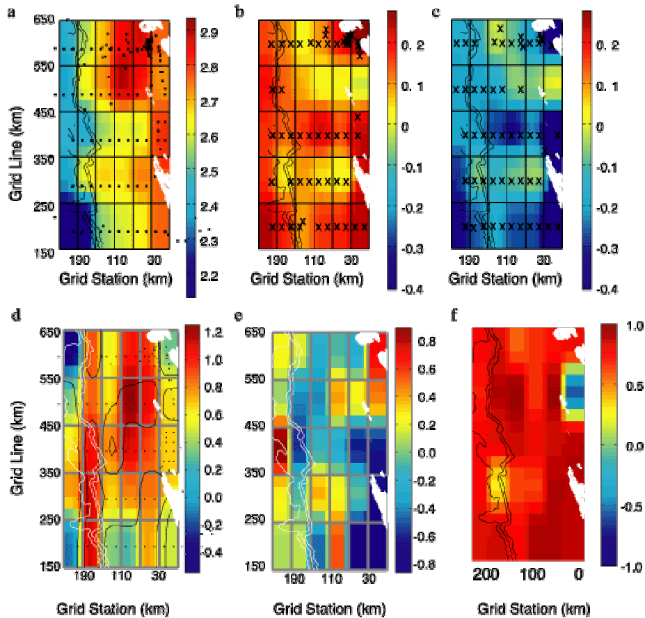
Fig. 2.16. a) Climatology of the log of primary production (PP, \text{mgC m}^{-2} \text{d}^{-1} ) for PAL January cruises, 1995-2000. b) interpolated anomaly fields for climatology in 1996. c) anomaly field for 1999. X's are stations for each year. d) Climatology as color map with std dev contours (0.6, 1.0, 1.4) of krill abundance. e) the r value for interpolated log PP correlated against interpolated krill abundance. f) heterogeneous correlation map (r value) of log PP on PC3 of krill abundance. Figures show land mass in white, 1000 m depth lines in gray, dots and x's mark data points and gray solid lines are cell borders used in gridding data.
