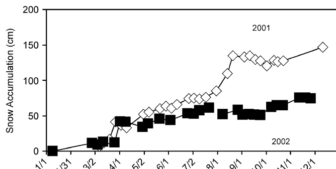
Fig. 3. Snow accumulation at Rothera Station measured during 2001 and 2002. (data courtesy of the meteorological monitoring team of the Rothera Station—British Antarctic Survey).
