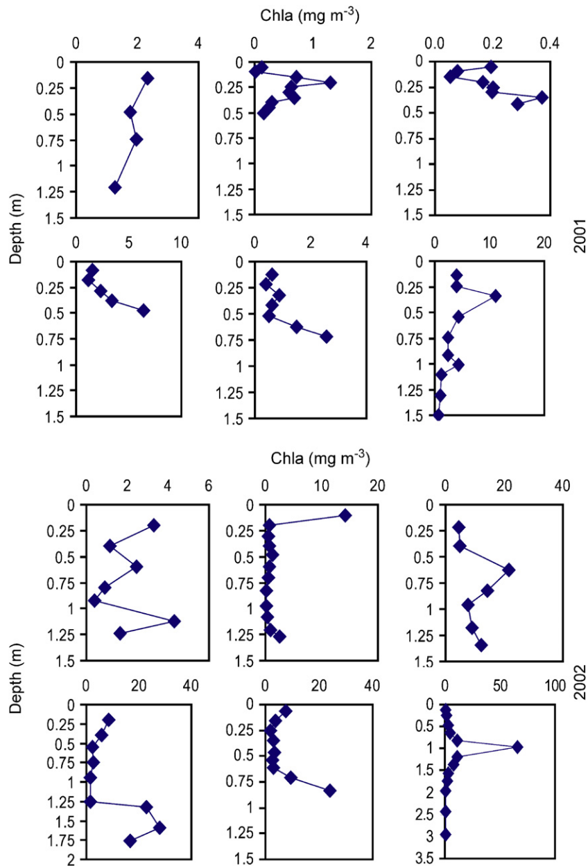
Fig. 7. Examples of the vertical profiles of chlorophyll a in ice cores from both 2001 and 2002 studies illustrating maxima occurring in bottom, middle, and surface sections of the ice floes. Note the differences in the scales for chl a concentrations among the ice cores.
