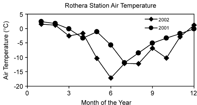
Fig. 2. Monthly averaged air temperatures at Rothera Station (British Antarctic Survey) during 2001 and 2002.
