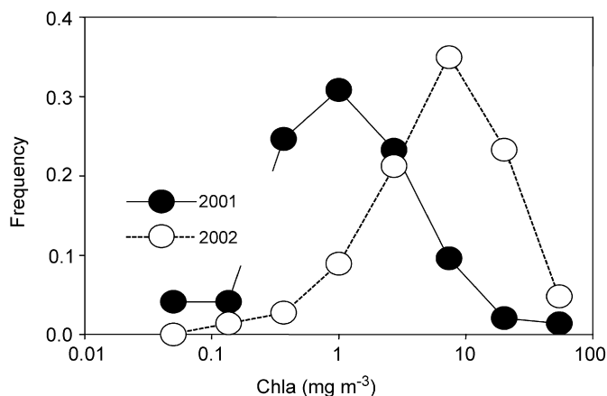
Fig. 8. Histogram of chlorophyll a content of ice cores that were collected at overlapping times of the year during 2001 and 2002 cruises.
