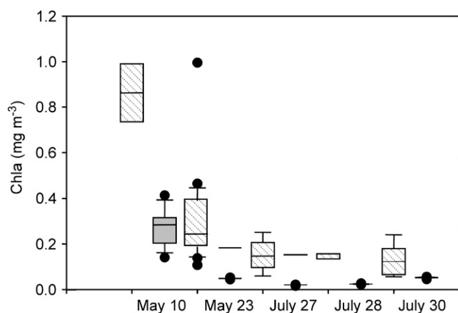
Fig. 6. Chlorophyll a concentrations in water collected in the upper 50 m of water column (gray boxes) and in newly formed ice (hatched boxes) collected at different times during the 2001 SO-GLOBEC cruises. Boxes show 65% confidence intervals while error bars denote 95% confidence intervals.
