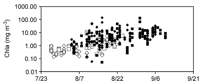
Fig. 9. Depth-averaged chlorophyll a content of ice cores collected during 2001 and 2002 shown in relation to the time (month/day) of the core collections. Open symbols denote 2001 samples and closed symbols represent those in 2002.
