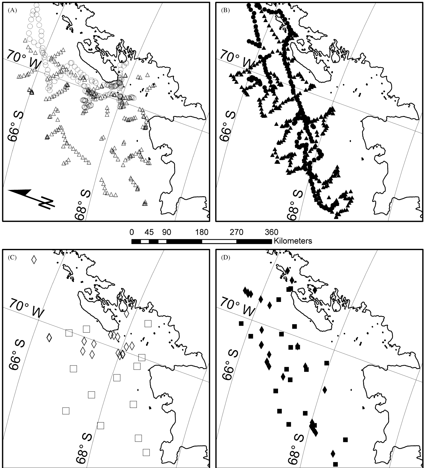
Fig. 1. Locations of ice observations (A and B) made during cruises on board the ARSV Lawrence M. Gould (circles) and RVIB Nathaniel B. Palmer (triangles) during 2001 (A) and 2002 (B). Locations where ice cores were taken are also shown (2001 \frac{1}{4} C, 2002 \frac{1}{4} D; NBP cores in squares and LMG cores in diamonds). For more information on cruises see http://www.ccpo.edu/Research/globec_menu.html and Hofmann et al. (2002).
