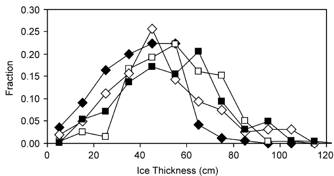
Fig. 5. Thickness distributions for ice observed from the LMG (diamonds) and NBP (squares) during GLOBEC cruises of 2001 (open symbols) and 2002 (closed symbols).
