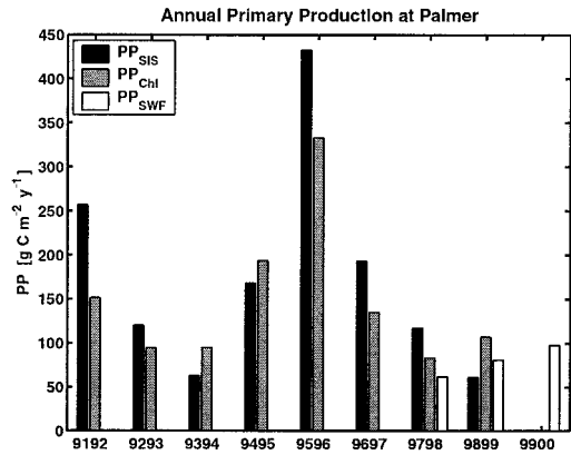
FIG. 6. Annual primary production (g C m -2 yr -1 ) determined near Palmer Station for each growing season from 1991/92 to 1999/2000. First, annual estimate have been made from integrated near-weekly surface sampling over the growing season from November to March (152 days) at Palmer Station (PP SIS ). Production determined as described in Figure 3. Second, annual production estimated based on Palmer Station chl-a measurements using our production model and integrated over the same growing season (PP CHL ). Third, estimates from modeled primary production based on average monthly chl-a retrieved from SeaWiFS ocean color data (for the three years the satellite has been in orbit) (PP SWF ).
