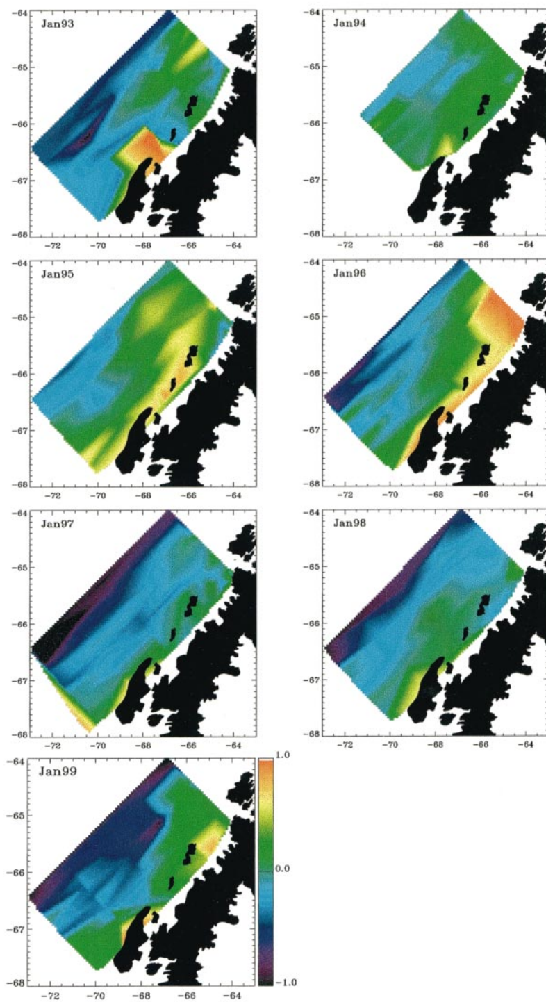
FIG. 4. Chl-a concentration (mg chl-a m -3 ) averaged within the euphotic zone in the Palmer LTER grid for each January cruise from 1993 to 1999.
