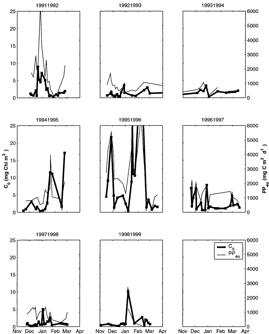
FIG. 3. Surface chl-a ( mg\ chl\ m^{-3} , thick line) and water column integrated primary production ( mg\ C\ m^{-2}\ day^{-1} , thin line). Data averaged for nearshore stations (B & E) and presented as a function of time during the growing season from 1991/92 through 1998/99. Data for the 1991/92 through 1993/94 season are estimated using photosynthesis irradiance curves integrated to 60 m (Moline and Prezelin, 1996). Data from 1994/95 through 1999/00 estimated from simulated in situ observations (SIS), as described in the text, integrated to the depth representing 2% of surface irradiance.
