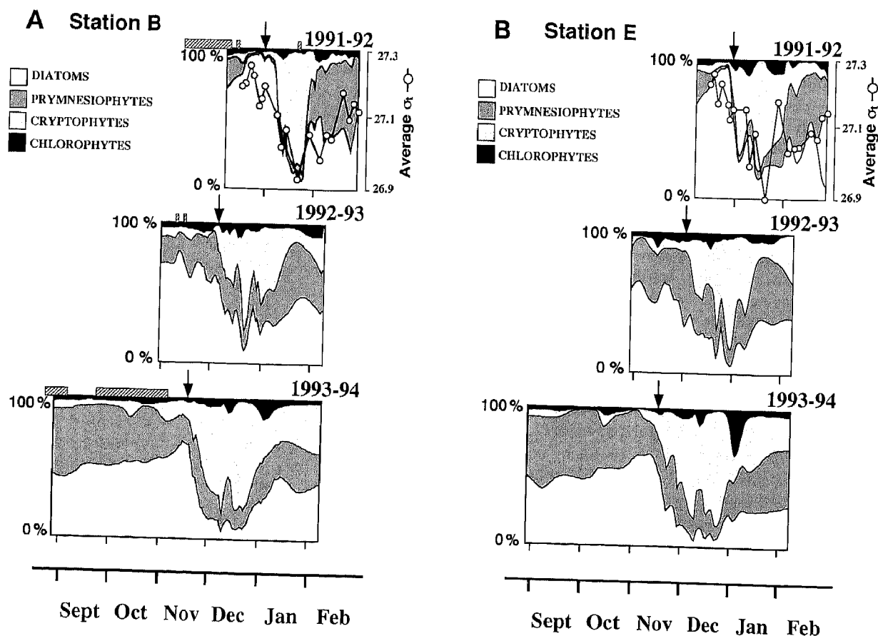
Fig. 9. Seasonal change in the depth integrated percent composition of the 4 different phytoplankton groups represented at (A) Stn B and (B) Stn E over the 3 field seasons from 1991 to 1994. Overlaid on the 1991-1992 panel is the change in the average water column density ( \sigma_t ) in the upper 50 m. The presence of significant fast/pack ice (>50% coverage) is indicated by hatch bars. Arrows are same as in Fig. 2A
