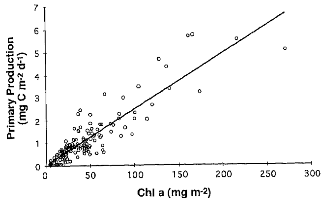
Fig. 8. Total integrated chl a in the euphotic zone (0.1% Q_{PAR} isolume) versus the daily simulated in situ production for Stns B and E over the 3 field seasons from 1991 to 1994. The best-fit linear regression is included [ P = 0.025 \times \text{Chl } a + 0.015 , r^2 = 0.80 , n = 156 ]
